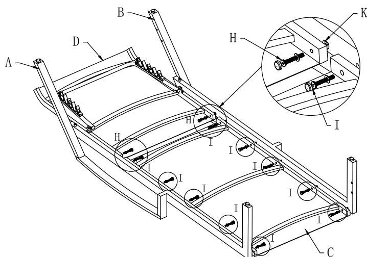
Lounge leg (A) X1
